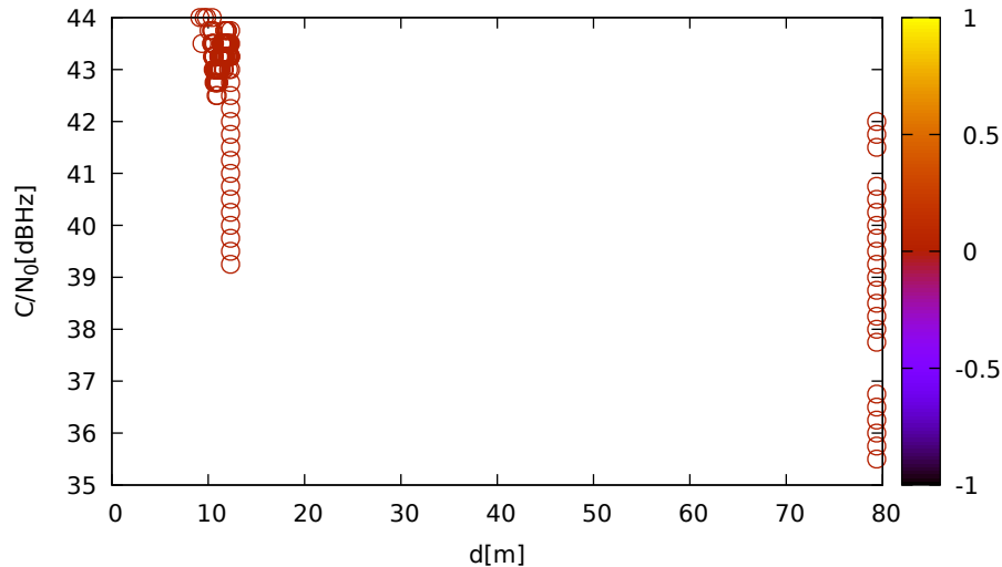
C/N 0 vs distance (JavadLSA at C 3 for E12 at L5)
