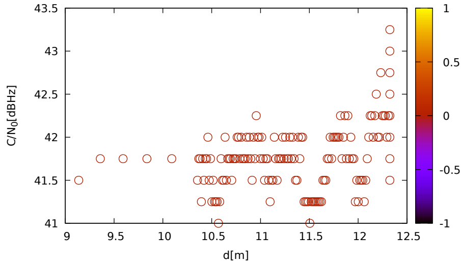
C/N 0 vs distance (JavadLSA at C 3 for E19 at L5)
