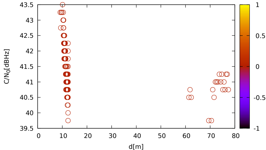
C/N 0 vs distance (JavadLSA at C 3 for E30 at L5)
