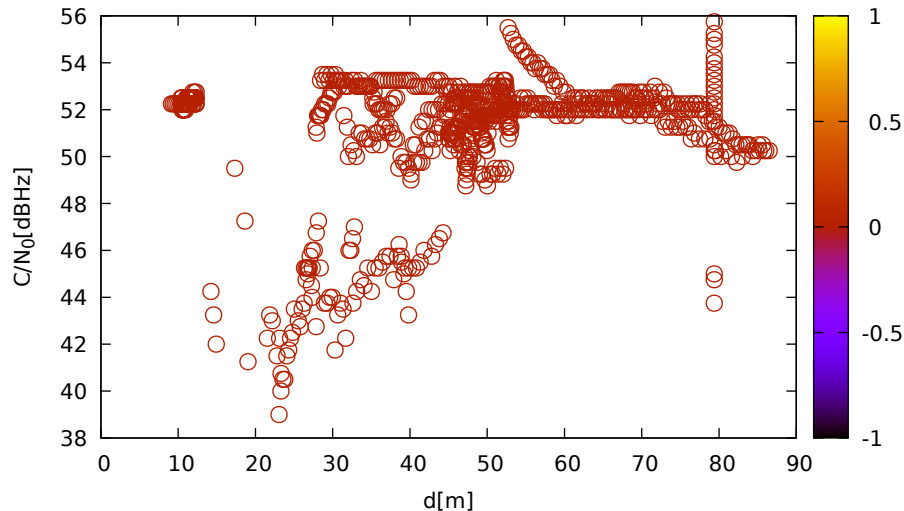
C/N 0 vs distance (JavadLSA at C 3 for E36 at L5)
