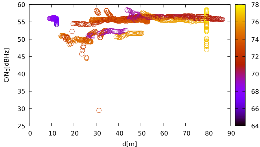
C/N 0 vs distance (JavadLSA at C 3 for G01 at L5)
