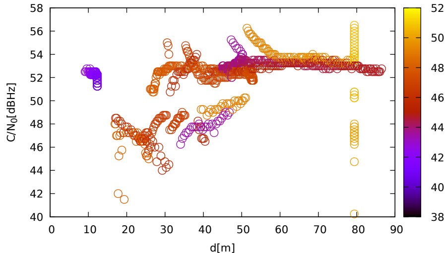
C/N 0 vs distance (JavadLSA at C 3 for G03 at L5)
