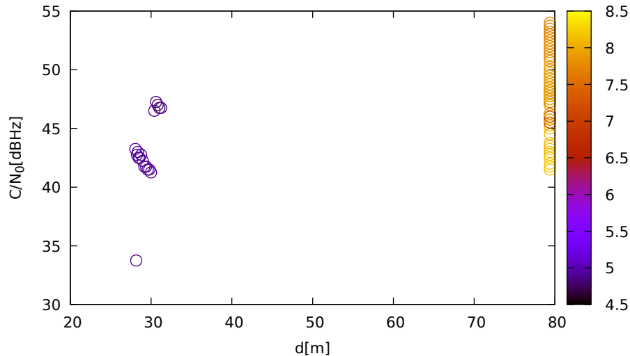
C/N 0 vs distance (JavadLSA at C 3 for G04 at L5)
