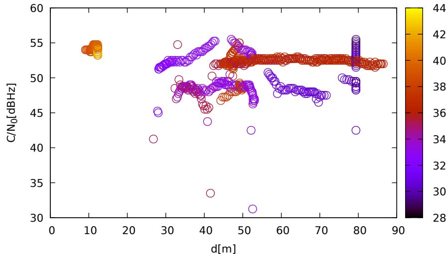
C/N 0 vs distance (JavadLSA at C 3 for G08 at L5)
