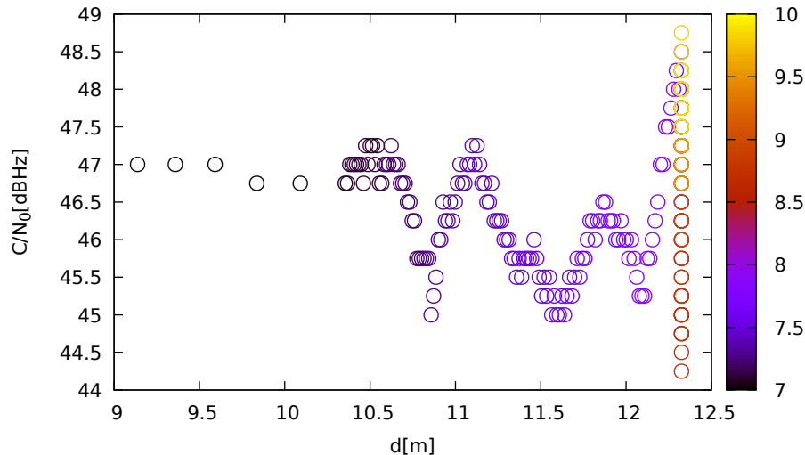
C/N 0 vs distance (JavadLSA at C 3 for G10 at L5)
