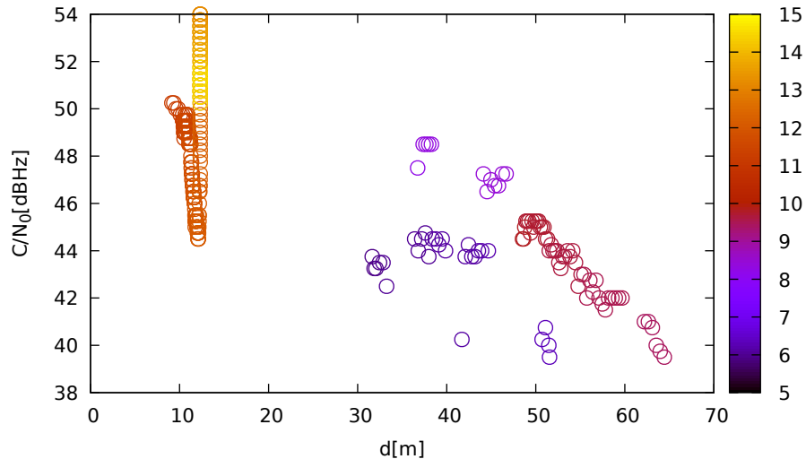
C/N 0 vs distance (JavadLSA at C 3 for G27 at L5)
