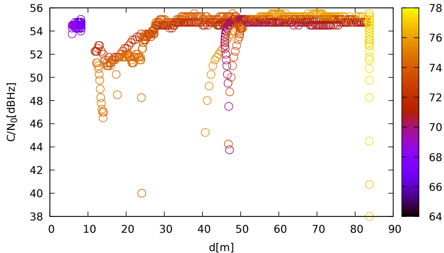
C/N 0 vs distance (JavadVS at C 3 for G01 at L5)
