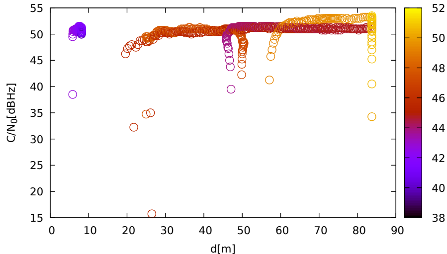
C/N 0 vs distance (JavadVS at C 3 for G03 at L5)
