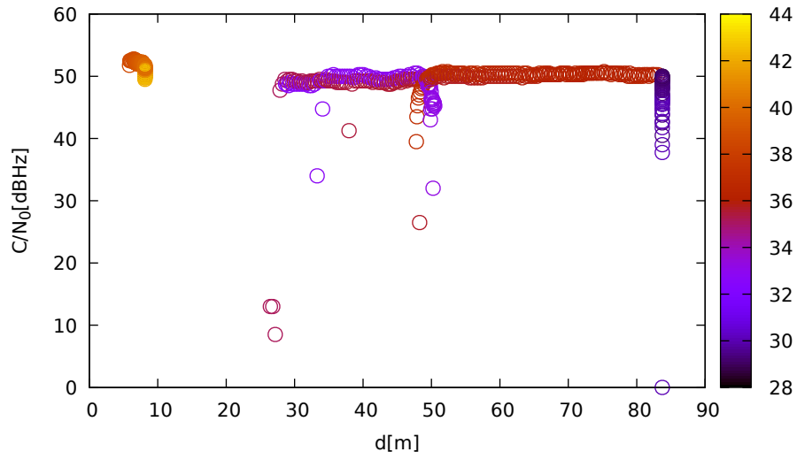
C/N 0 vs distance (JavadVS at C 3 for G08 at L5)
