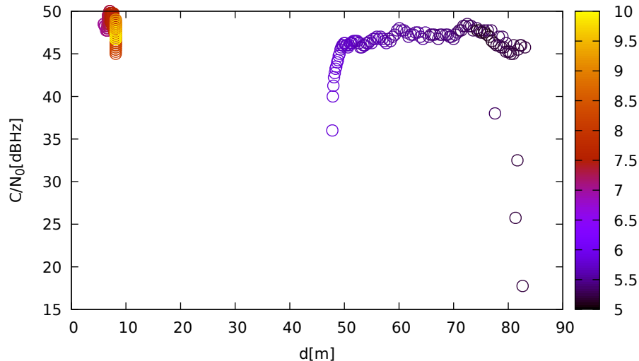
C/N 0 vs distance (JavadVS at C 3 for G10 at L5)
