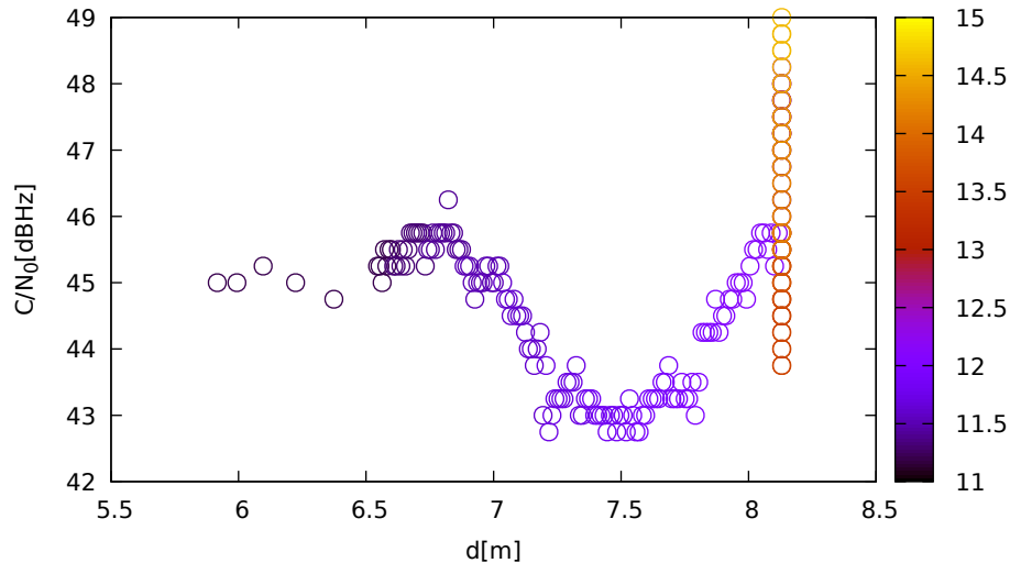
C/N 0 vs distance (JavadVS at C 3 for G27 at L5)
