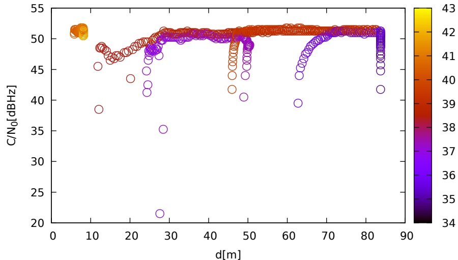
C/N 0 vs distance (JavadVS at C 3 for G32 at L5)
