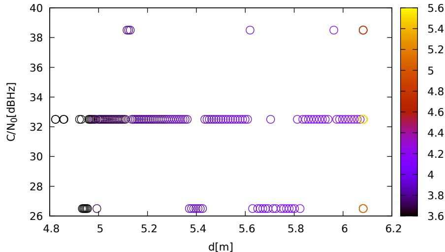
C/N 0 vs distance (LeicaGS15 at C 3 for E02 at L5)
