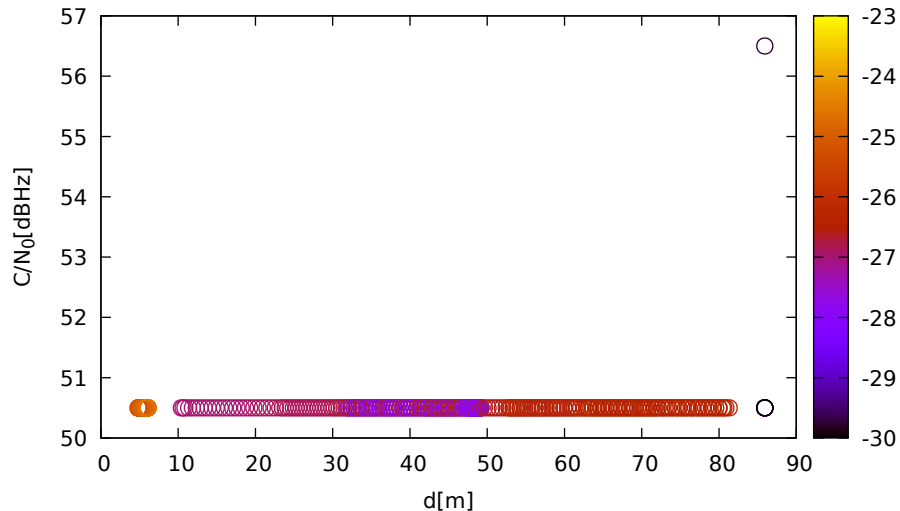
C/N 0 vs distance (LeicaGS15 at C 3 for E04 at L5)
