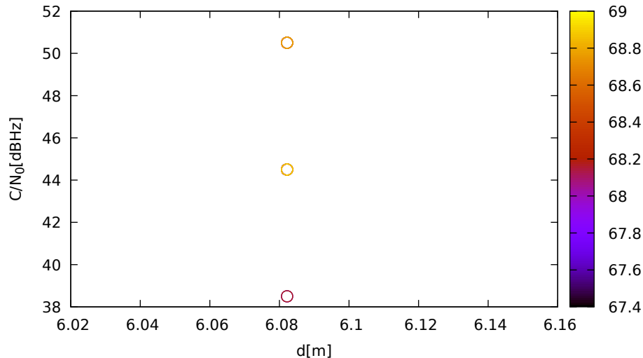
C/N 0 vs distance (LeicaGS15 at C 3 for E05 at L5)
