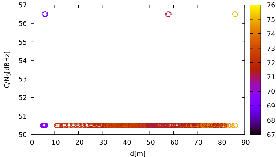
C/N 0 vs distance (LeicaGS15 at C 3 for E09 at L5)
