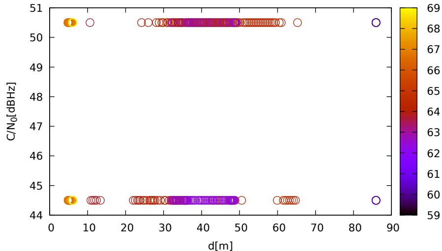
C/N 0 vs distance (LeicaGS15 at C 3 for E11 at L5)
