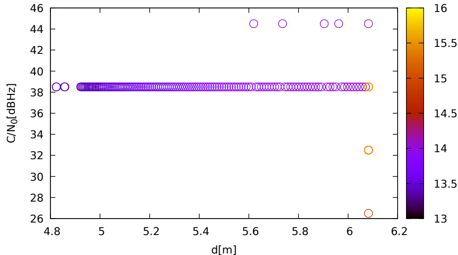
C/N 0 vs distance (LeicaGS15 at C 3 for E12 at L5)
