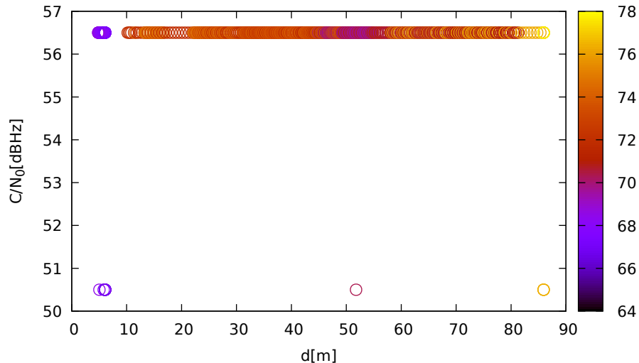
C/N 0 vs distance (LeicaGS15 at C 3 for G01 at L5)
