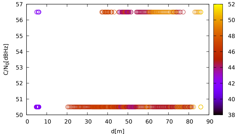
C/N 0 vs distance (LeicaGS15 at C 3 for G03 at L5)
