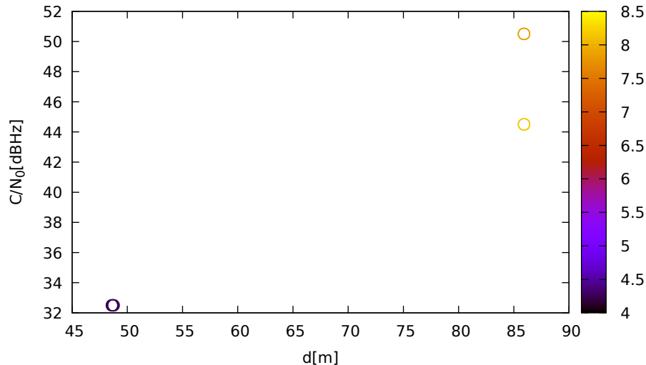
C/N 0 vs distance (LeicaGS15 at C 3 for G04 at L5)
