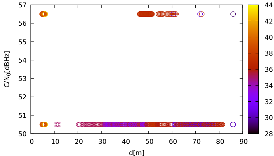
C/N 0 vs distance (LeicaGS15 at C 3 for G08 at L5)
