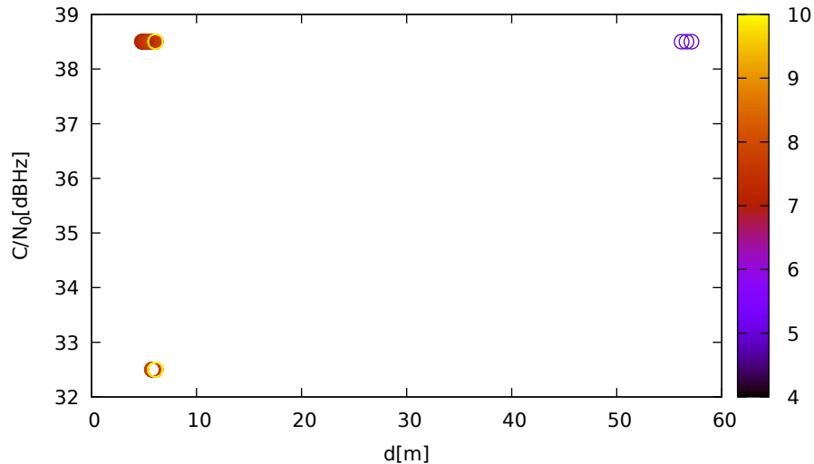
C/N 0 vs distance (LeicaGS15 at C 3 for G10 at L5)
