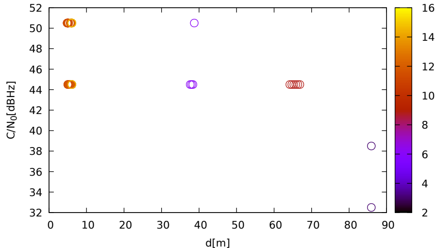
C/N 0 vs distance (LeicaGS15 at C 3 for G27 at L5)
