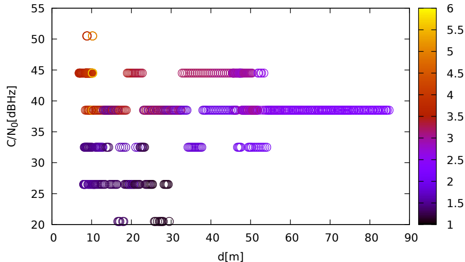
C/N 0 vs distance (LeicaGS18 at C 3 for E02 at L5)
