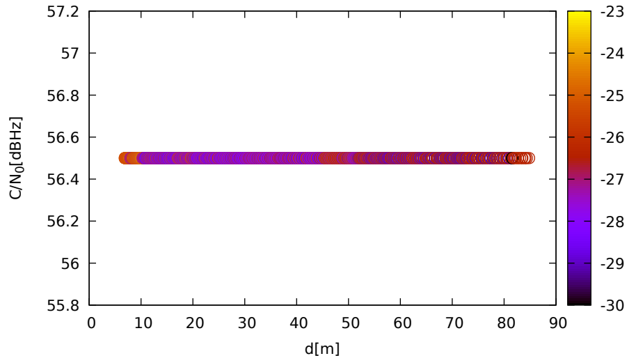
C/N 0 vs distance (LeicaGS18 at C 3 for E04 at L5)
