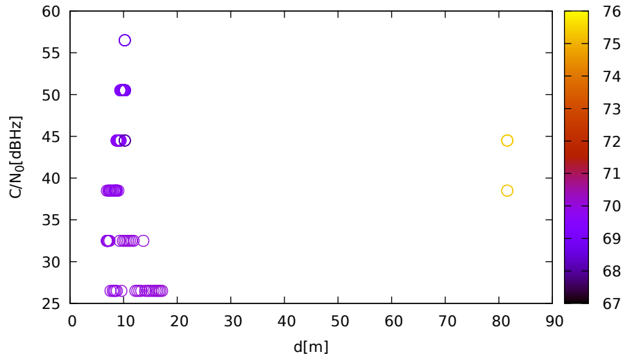
C/N 0 vs distance (LeicaGS18 at C 3 for E05 at L5)
