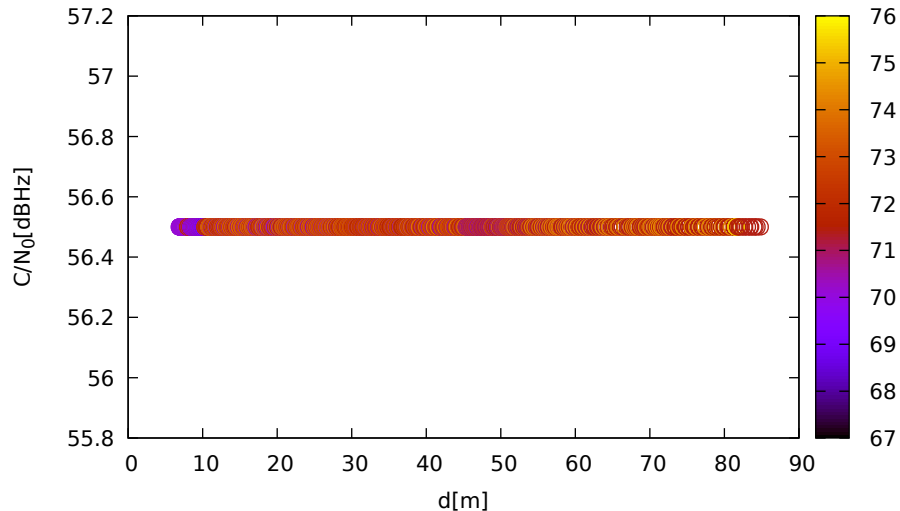
C/N 0 vs distance (LeicaGS18 at C 3 for E09 at L5)
