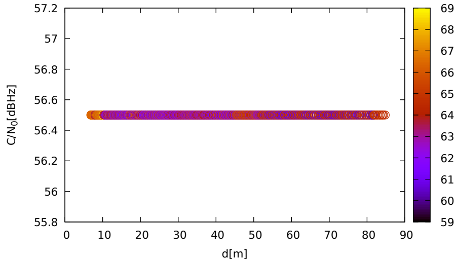
C/N 0 vs distance (LeicaGS18 at C 3 for E11 at L5)
