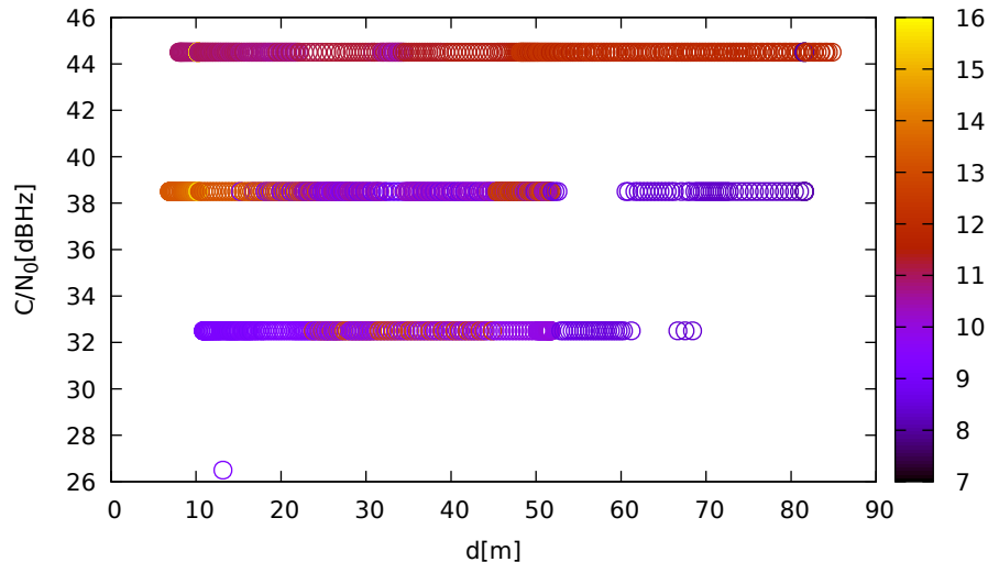
C/N 0 vs distance (LeicaGS18 at C 3 for E12 at L5)
