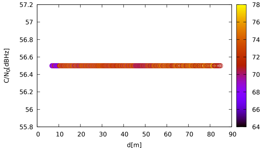
C/N 0 vs distance (LeicaGS18 at C 3 for G01 at L5)
