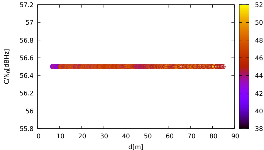
C/N 0 vs distance (LeicaGS18 at C 3 for G03 at L5)
