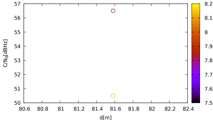
C/N 0 vs distance (LeicaGS18 at C 3 for G04 at L5)
