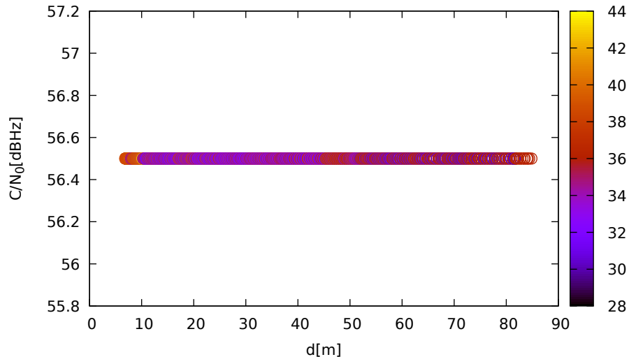
C/N 0 vs distance (LeicaGS18 at C 3 for G08 at L5)
