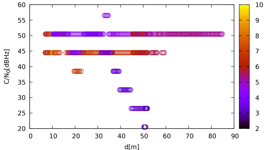
C/N 0 vs distance (LeicaGS18 at C 3 for G10 at L5)
