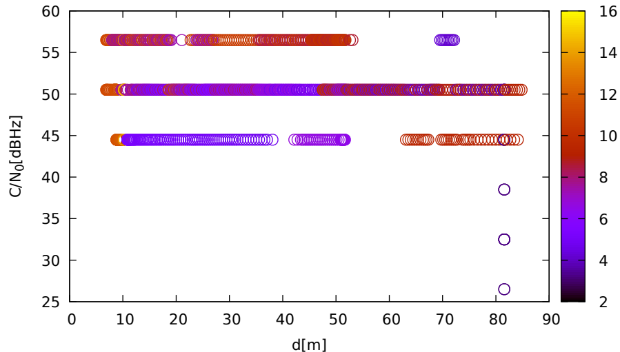
C/N 0 vs distance (LeicaGS18 at C 3 for G27 at L5)
