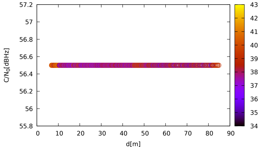
C/N 0 vs distance (LeicaGS18 at C 3 for G32 at L5)
