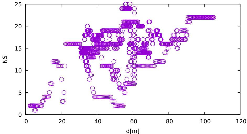
No. of satellites vs distance (LeicaGS15 at C_1 )
