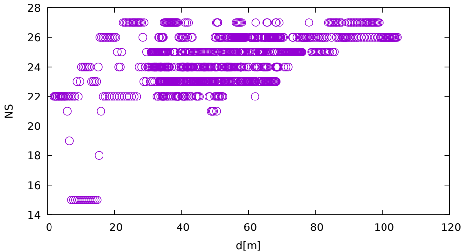
No. of satellites vs distance (LeicaGS18 at C 1 )
