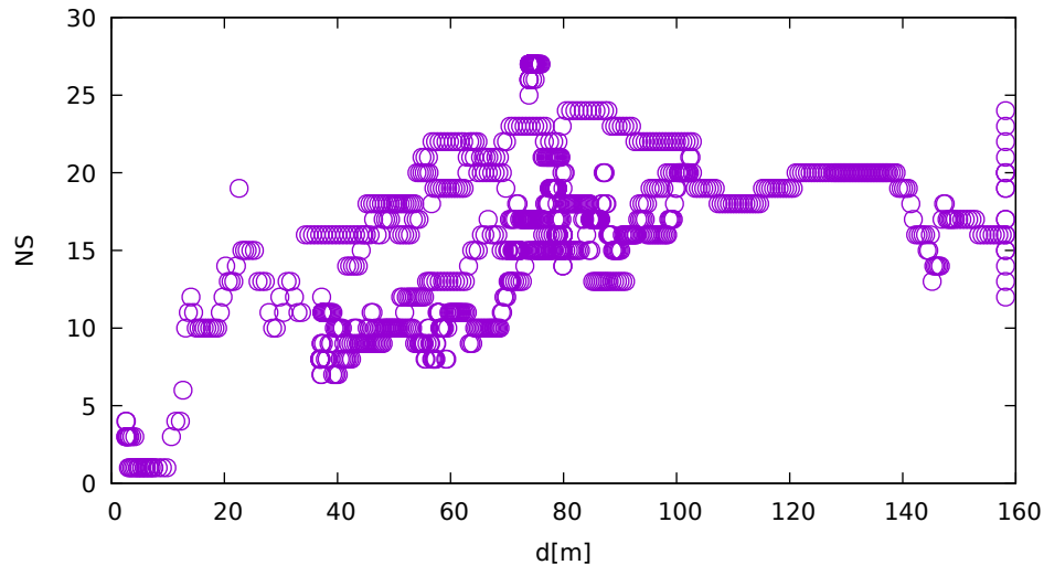
No. of satellites vs distance (LeicaGS15 at C 2 )
