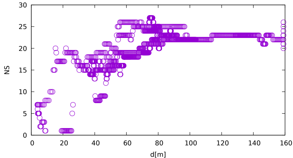
No. of satellites vs distance (TrimbleR10 at C 2 )
