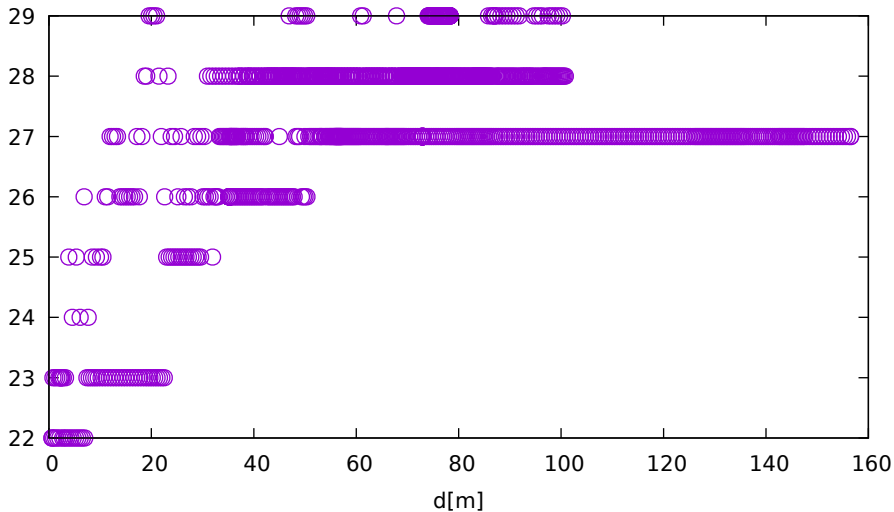
No. of satellites vs distance (ublox9 at C 2 )
