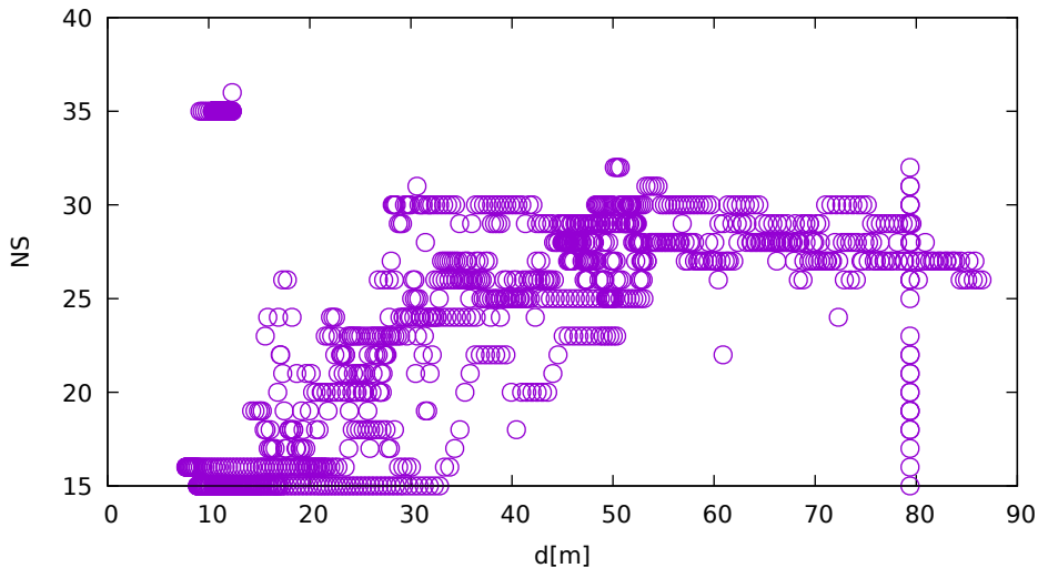
No. of satellites vs distance (JavadLSA at C 3 )
