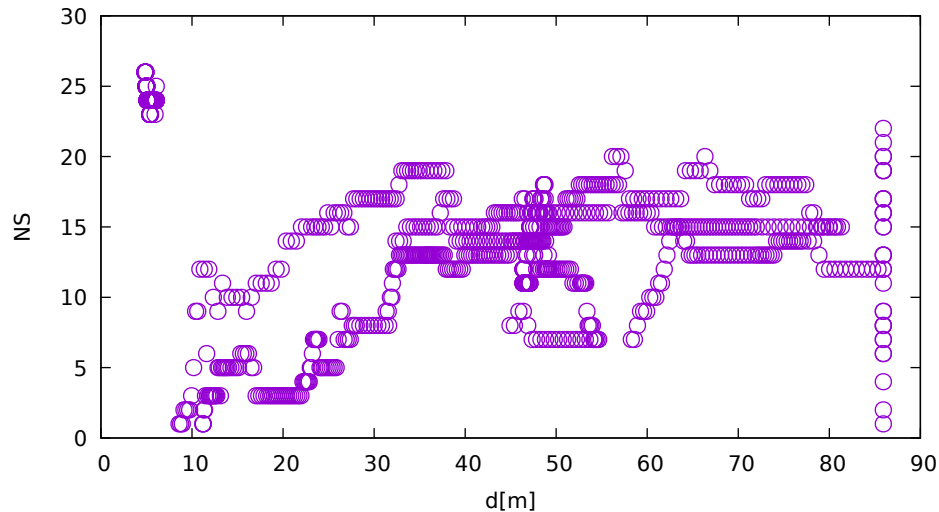
No. of satellites vs distance (LeicaGS15 at C 3 )
