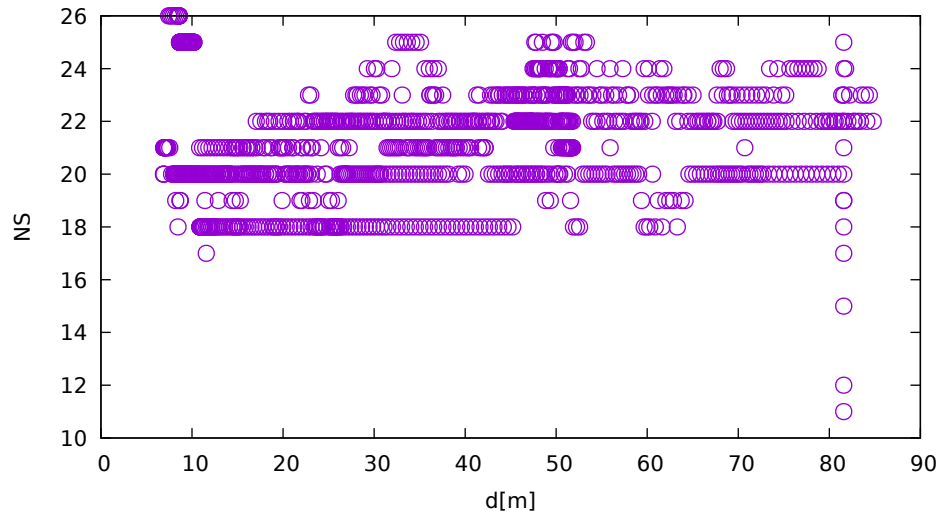
No. of satellites vs distance (LeicaGS18 at C 3 )
