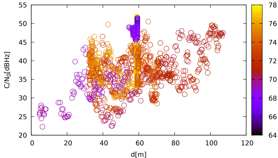
C/N 0 vs distance (JavadLSA at C 1 for G01 at L1)
